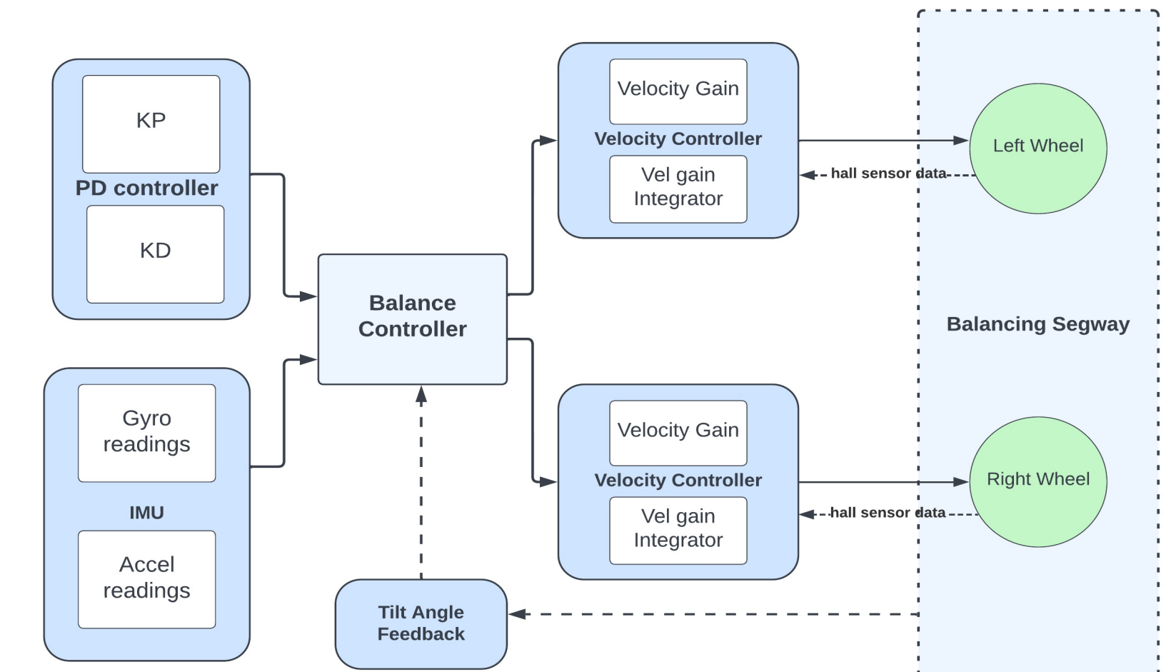
Figure 5: Control system block diagram for sensing and stabilization
